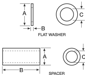
Washers/Spacers
