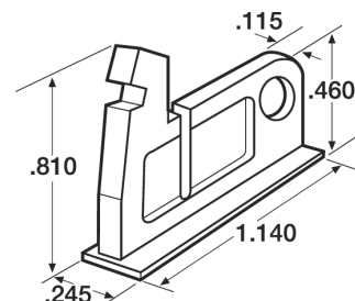
Latch
